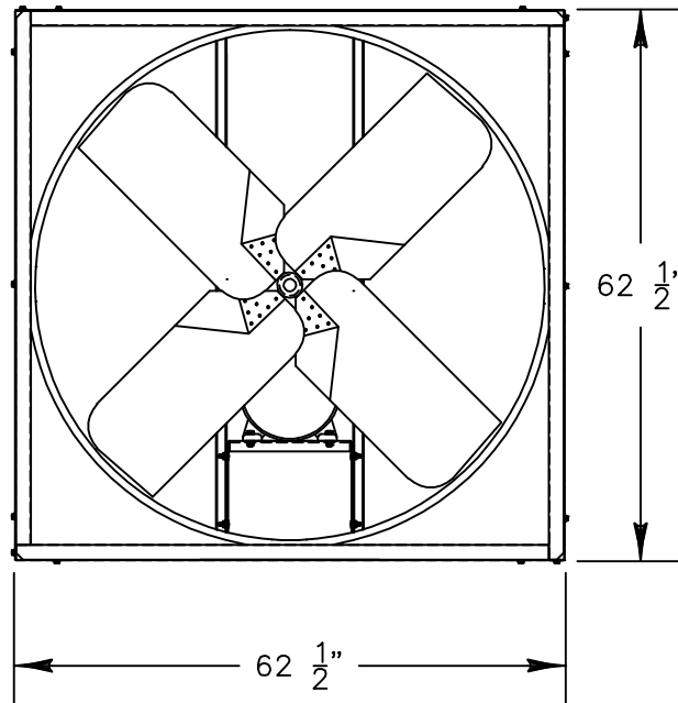
DISCHARGE VIEW
