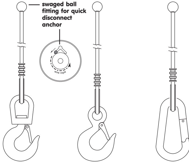
Swivel Hook
