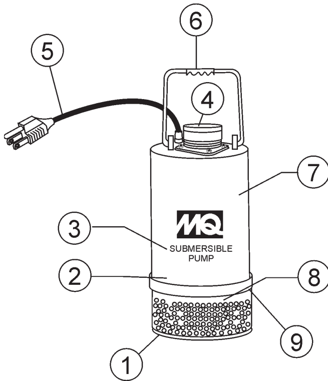
Figure 2. Submersible Pump Components
