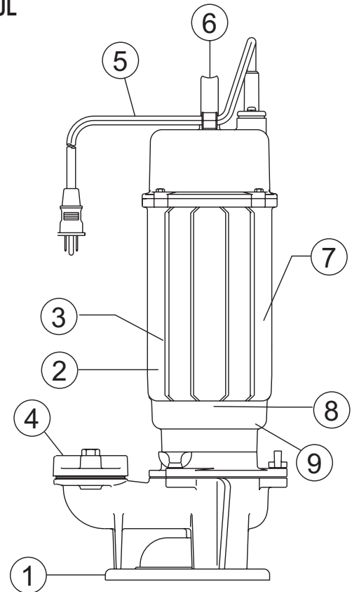
Figure 2. Submersible Pump Components
