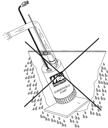
Figure 10. Submersible Pump Upright Position (Incorrect)
