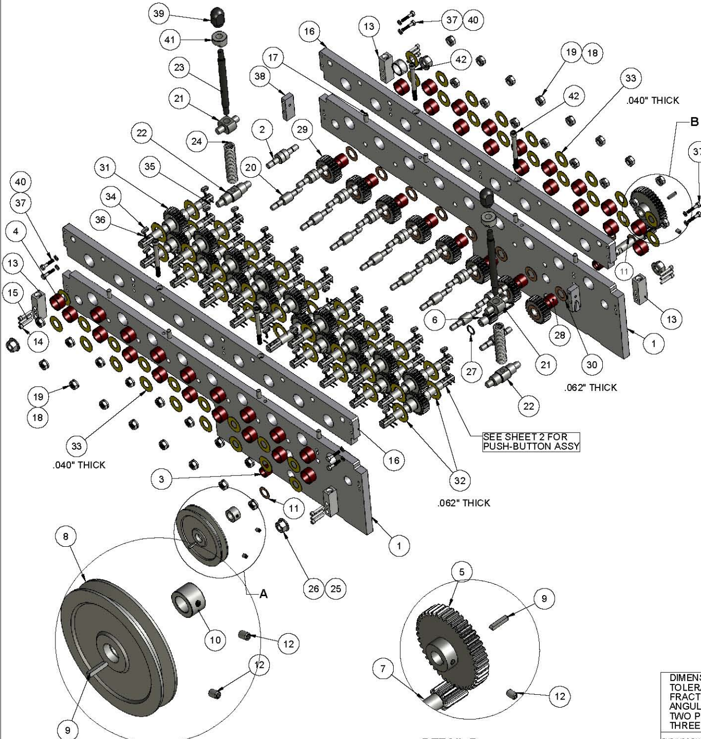
DETAIL A
