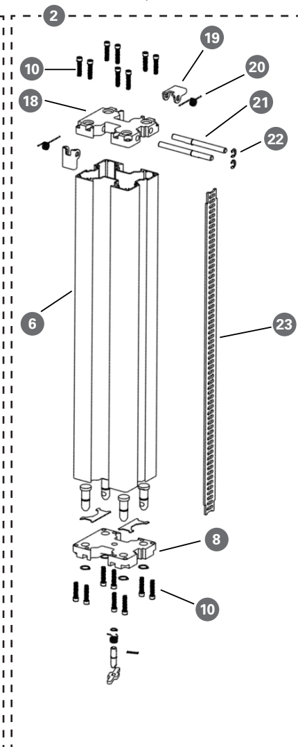
Middle Mast Assembly
