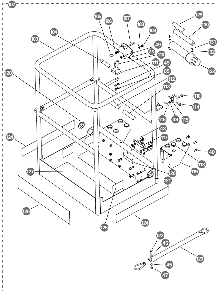
Platform Assembly
