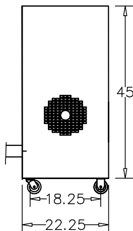
Right View
