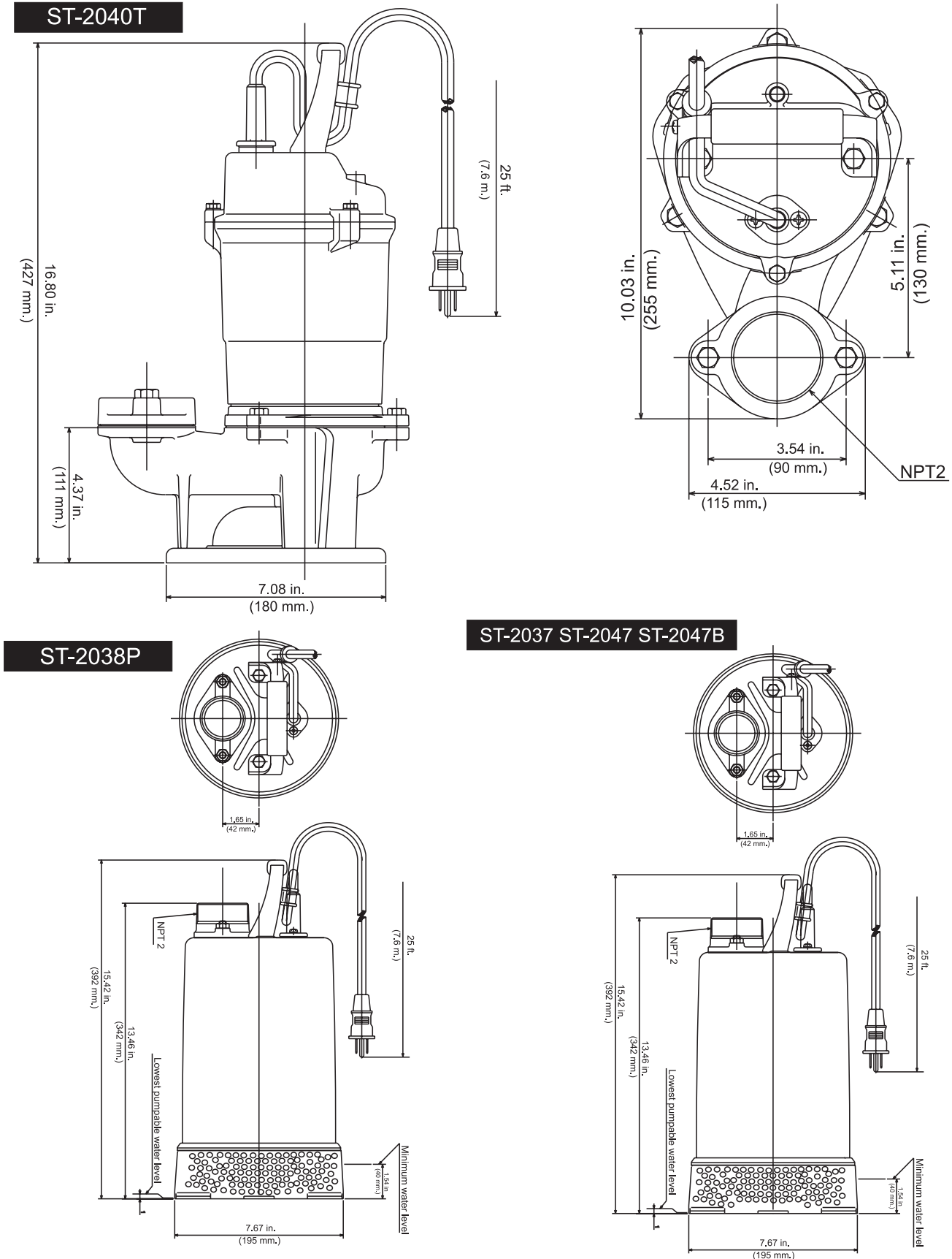
Figure 1. Submersible Pump Dimensions
