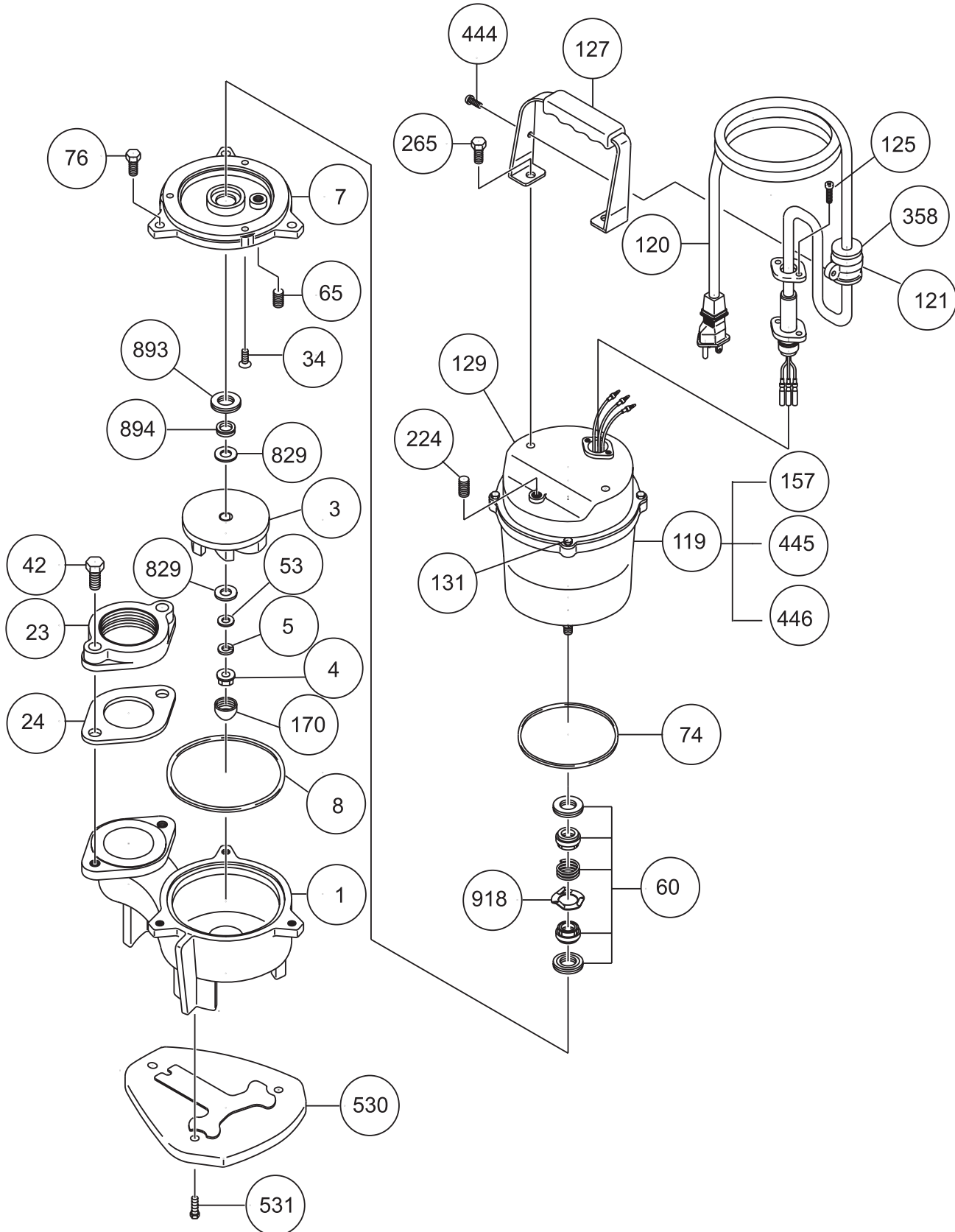
ST-2040T ELECTRIC SUBMERSIBLE PUMP ASSY.
